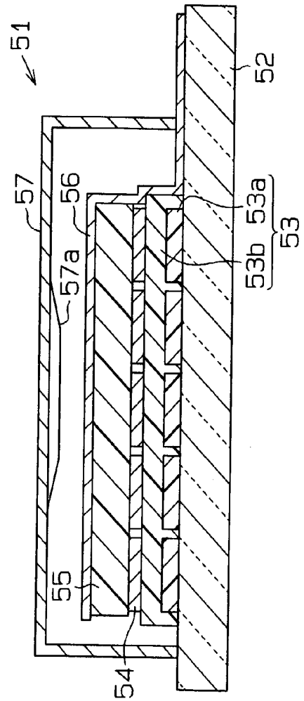
Fig. 4 (Prior Art)
